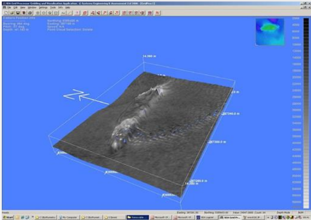
Side scan view of wreck (combine with 3D bathymetric data)
